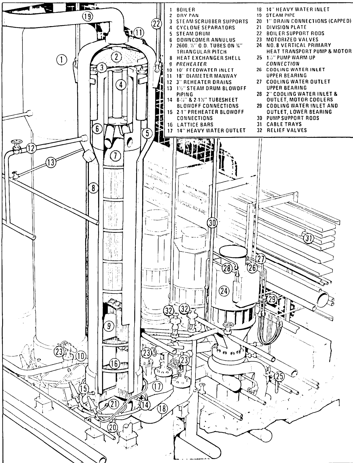
FIG. 7.4: Isometric view of boiler and pump arrangement.
