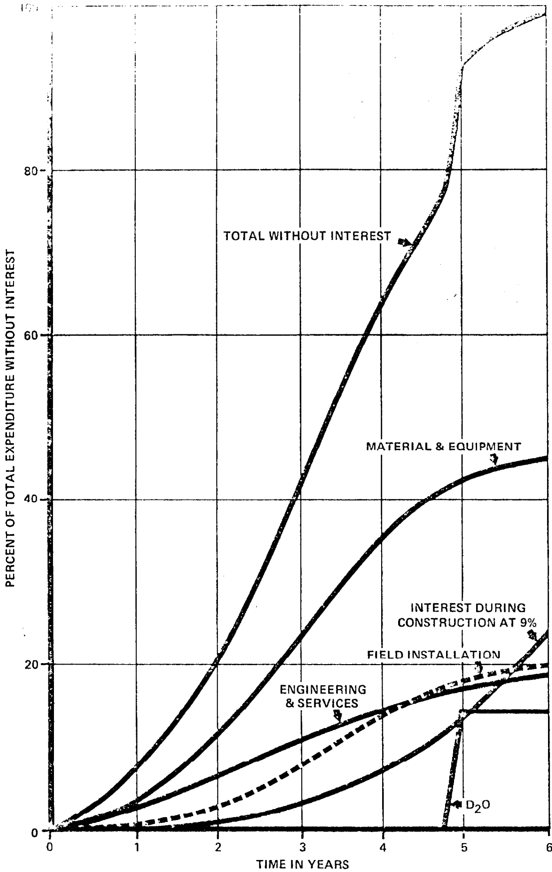
Fig. 10.20: Single Unit 600 MWe CANDU-PHW Plant Cash Flow
