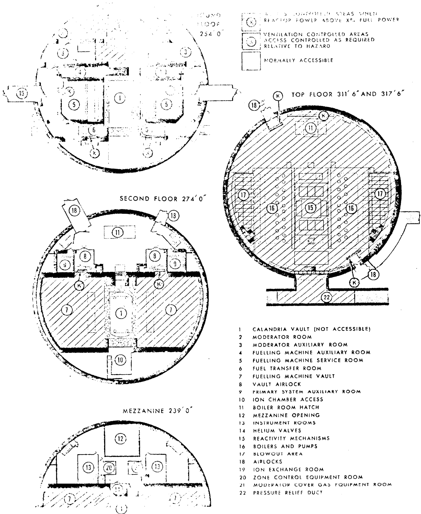
Fig. 10.13: Pickering G.S. - Reactor Building Access Control Diagram
