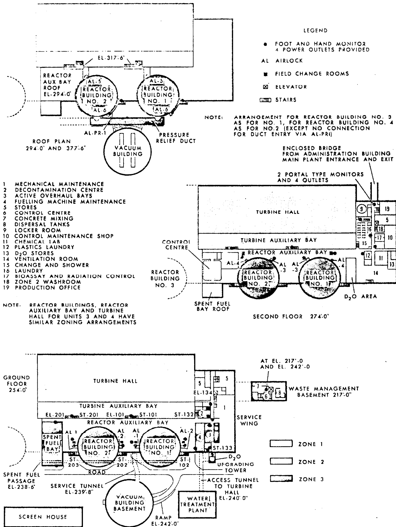
Fig. 10.14: Pickering G.S. - Plant Zoning Arrangement
