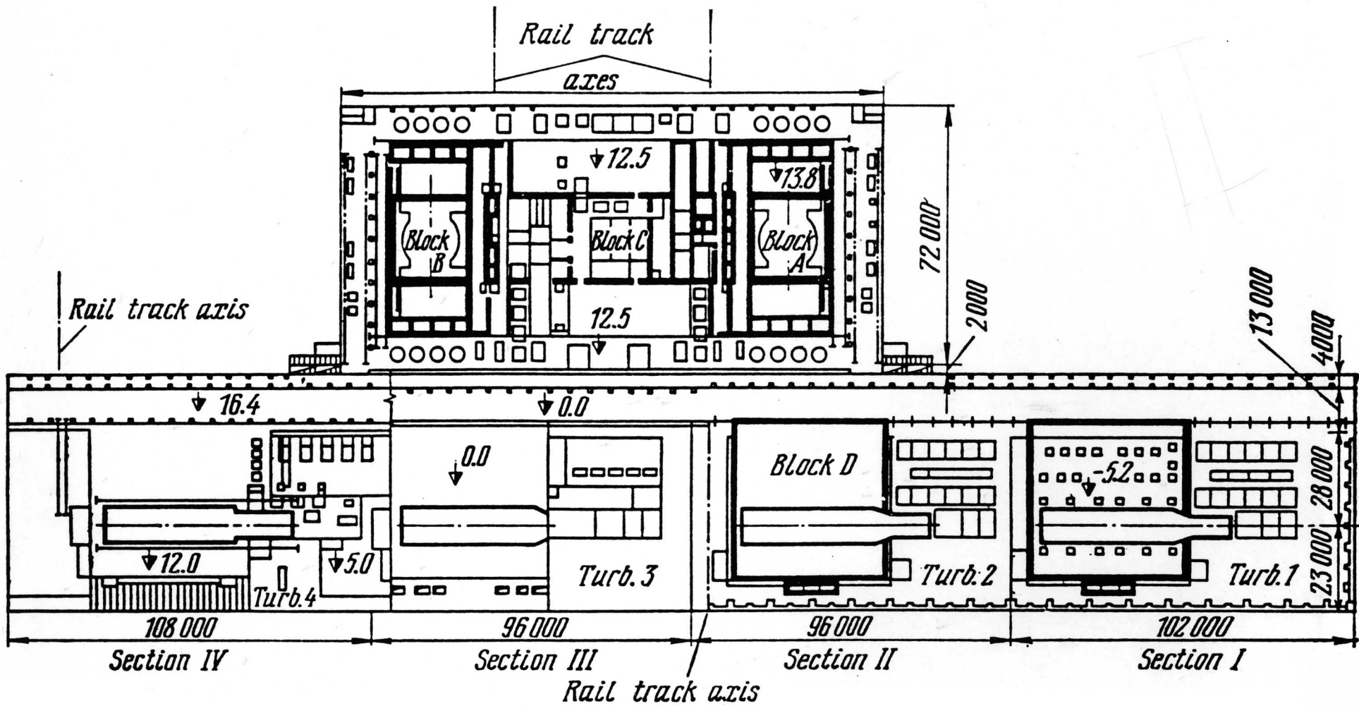
Plan of the main building at Smolensk
